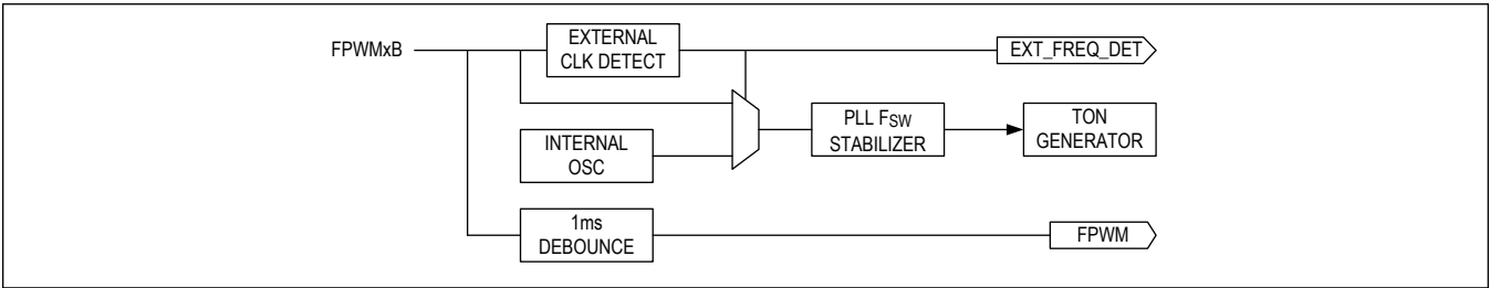
Figure 5. Frequency Tracking
