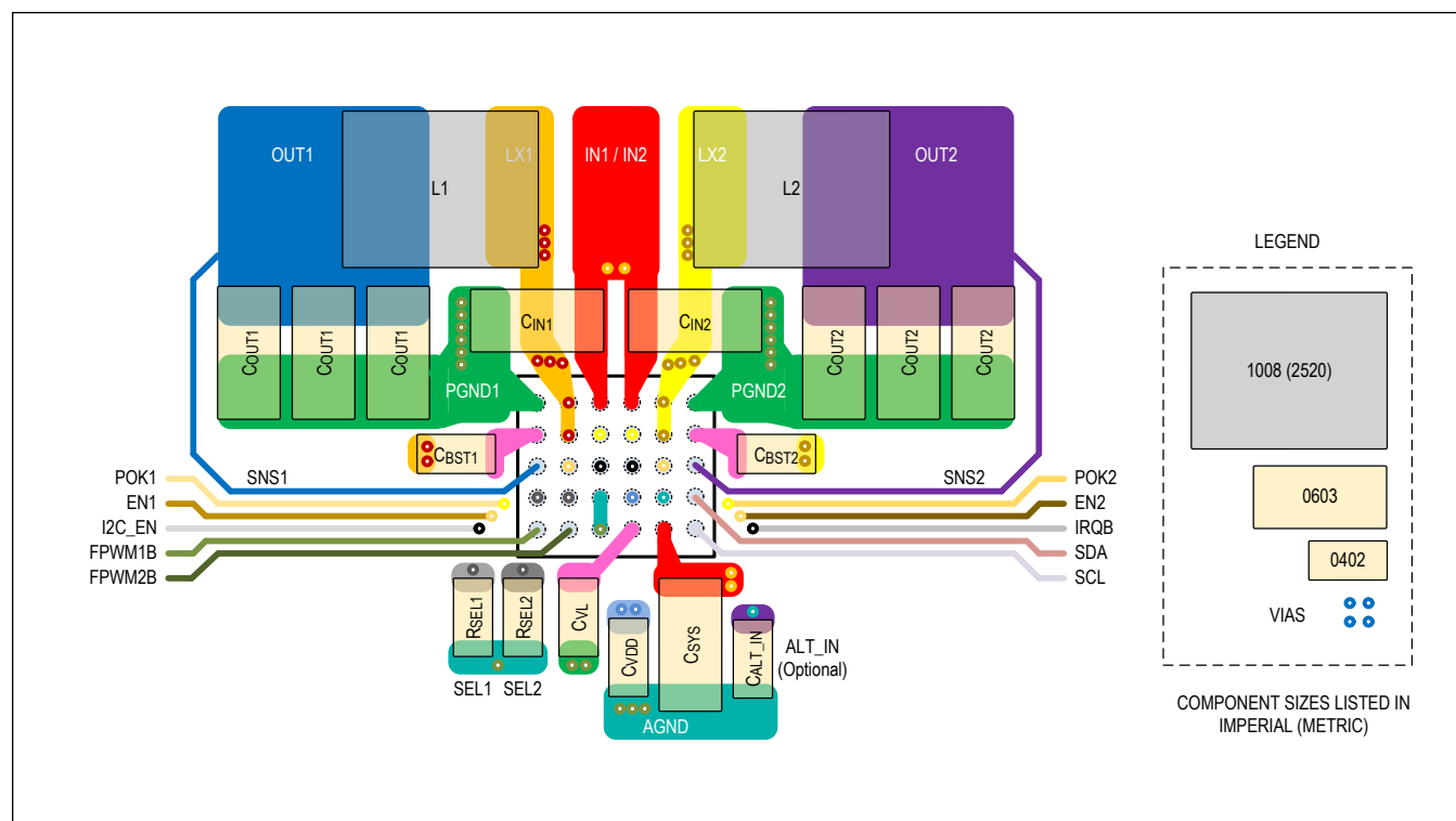
Figure 11. PCB Layout Example - WLP
